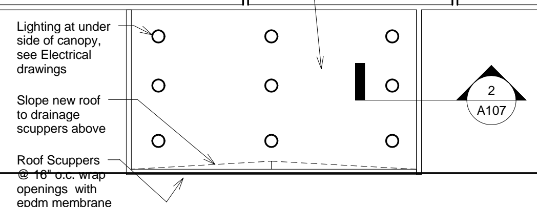
1 Reflected Ceiling Plan - North 1/8" = 1'-0"
