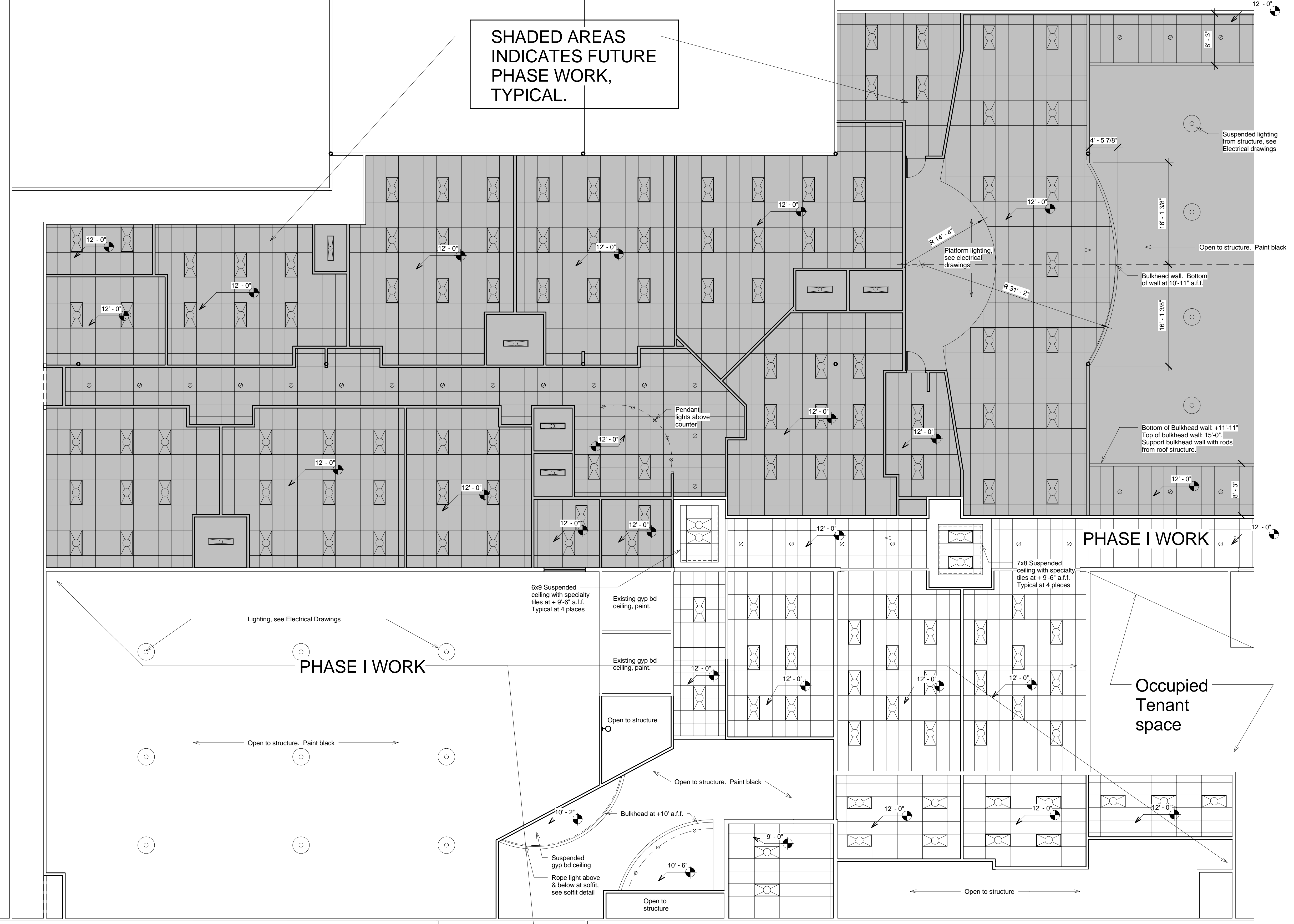
1 Reflected Ceiling Plan - North 1/8" = 1'-0"
