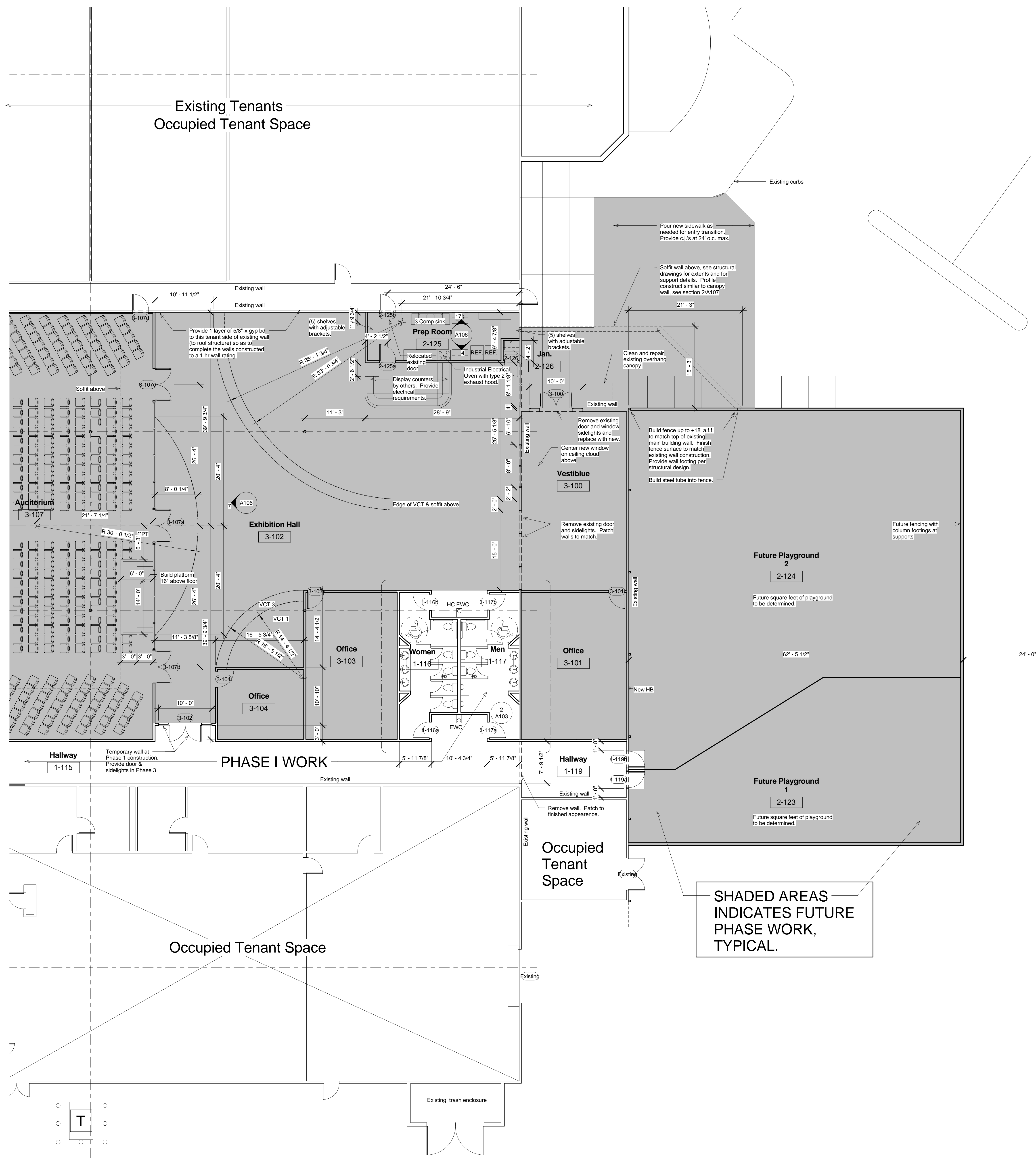
1 Floor Plan - South 1/8" = 1'-0"
