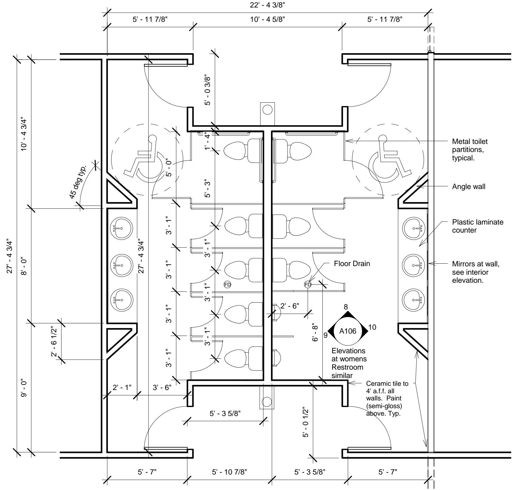
2 Enlarged Restroom Plan 1/4" = 1'-0"
